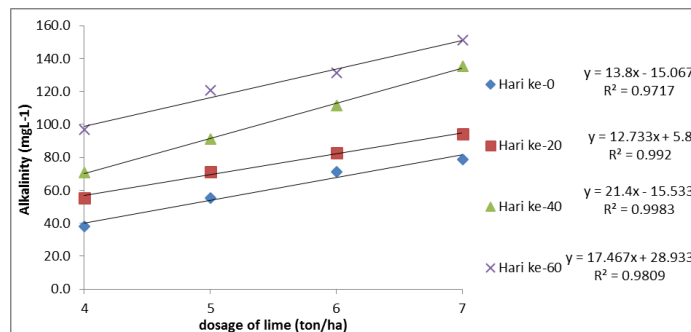
Fig 2. Relationship between dosage of lime and alkalinity
